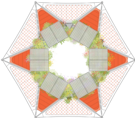
NIVEL DE PANELES SOLARES +36'-1 1/8" [11 m]
